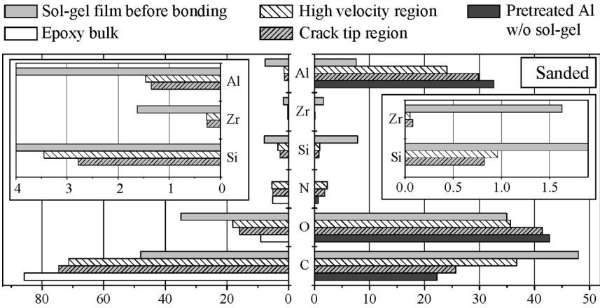
(c) Epoxy side ← Atomic Percentage, % → Aluminum side
